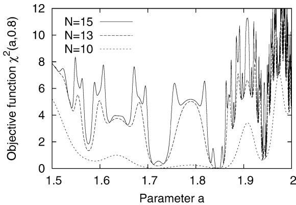
Fig. 1. Objective function of the logistic map Eq. (5) for noiseless data of different lengths N . For each length one time series was simulated with the true parameters \theta = (x_0, a) = (0.8, 1.85) and without noise. Then \chi^2(\theta) was plotted as a function of a , x_0 being set to its true value. Curves for higher N are higher than those for smaller N since the summands of Eq. (4) are non-negative. The global minimum at a = 1.85 becomes successively sharper but the number of local minima increases.
